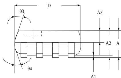
SOP8(W) PACKAGE OUTLINE DIMENSIONS
