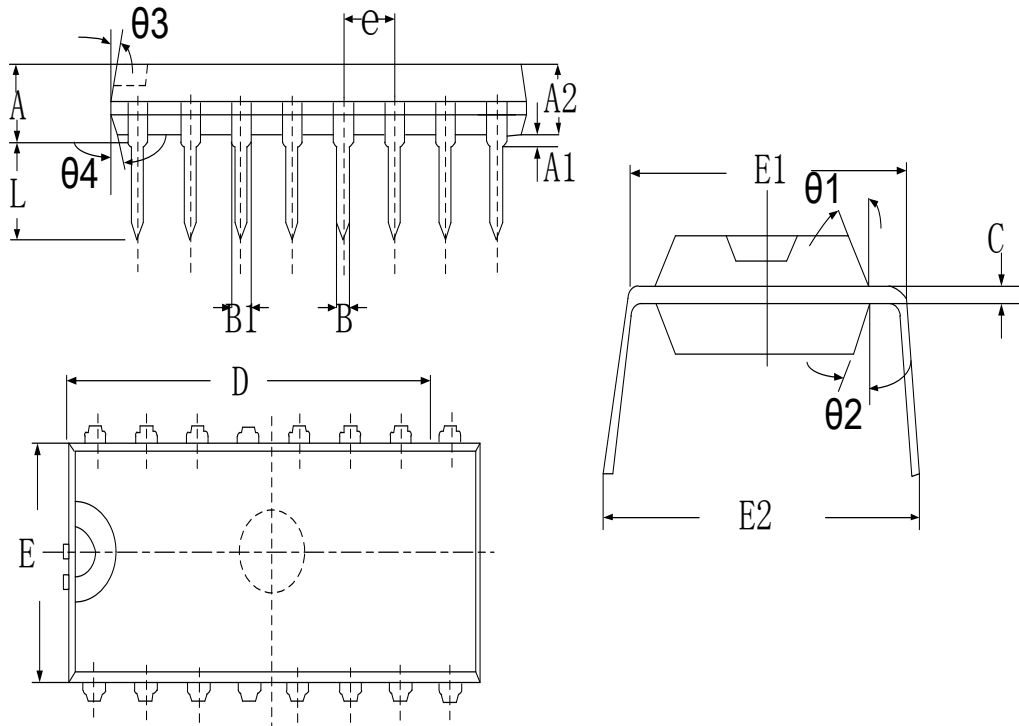
DIP16 PACKAGE OUTLINE DIMENSIONS
