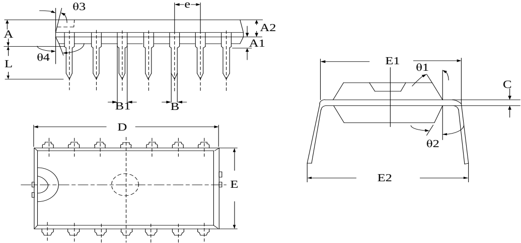
DIP14 PACKAGE OUTLINE DIMENSIONS
